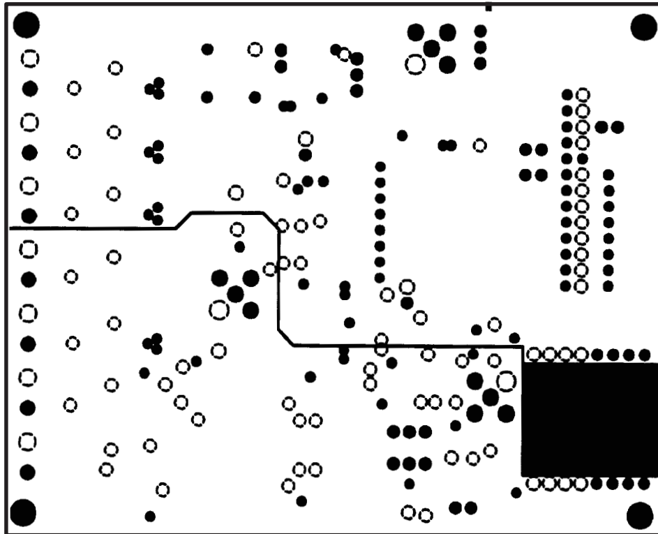
Internal Plane 1
